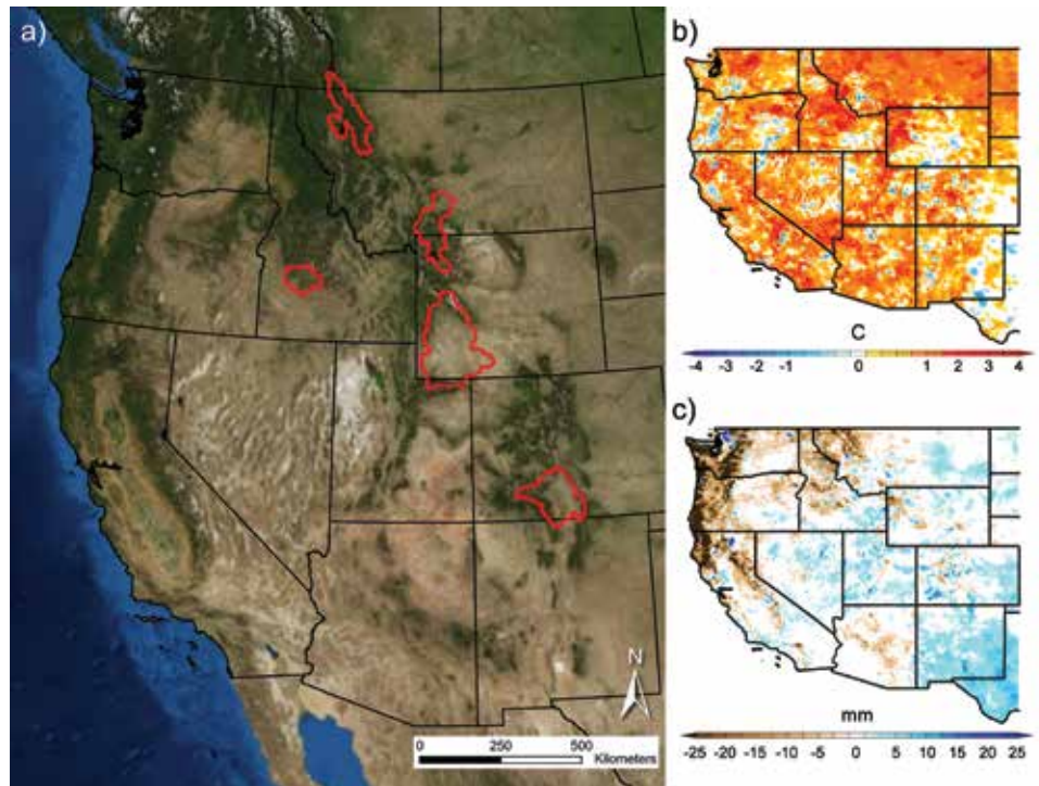
Figure 1. (a) Locations of case history areas examined to describe historical effects of climate change on trout streams across the Rocky Mountains. Change in (b) mean annual air temperature and (c) precipitation from 1950 to 2009. Mapped anomalies are the differences between averages for 1950–1959 and 2000–2009 based on PRISM data that were interpolated from climate monitoring stations (Daly et al. 1994).
