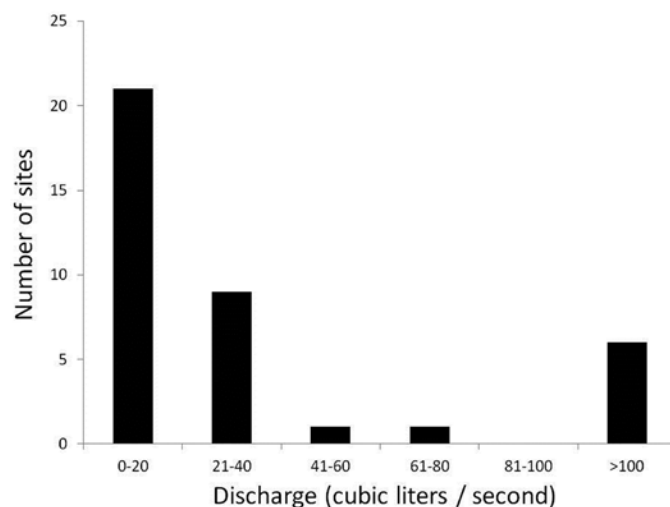
Figure 7. Frequency histogram showing the discharge in streams containing conservation populations of cutthroat trout in the Rio Grande during base flows in 2011 (n = 38). Measurement sites include mainstems near termini, important tributaries, and mainstems below the influence of important tributaries.
